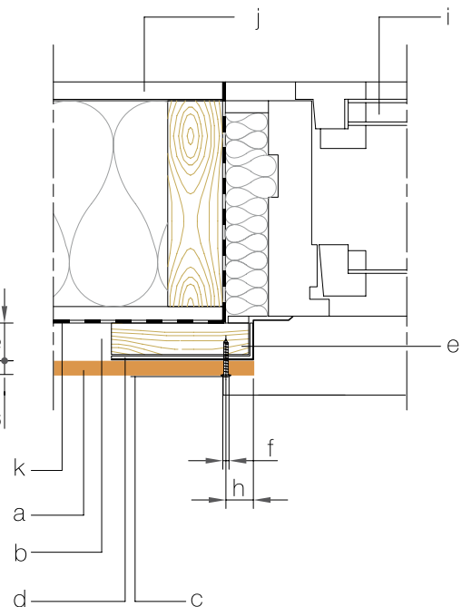
Figure 1 Window detail
